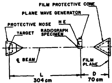
Fig 34 Experimental geometry
